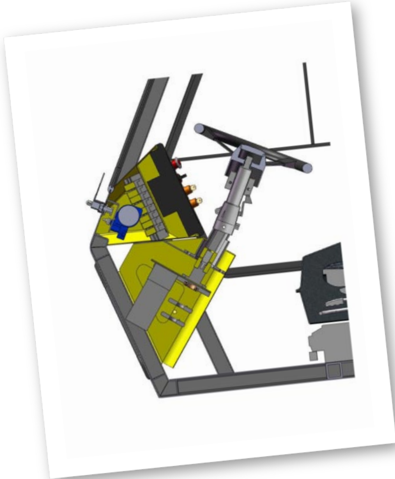
Cab Enclosure Steering Control assembly
